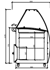
Side Drawing
